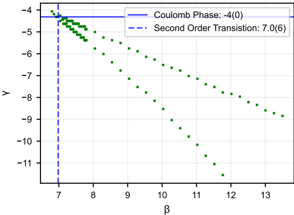
A5 Phase Diagram for Adjoint rep 5^{(0)}
